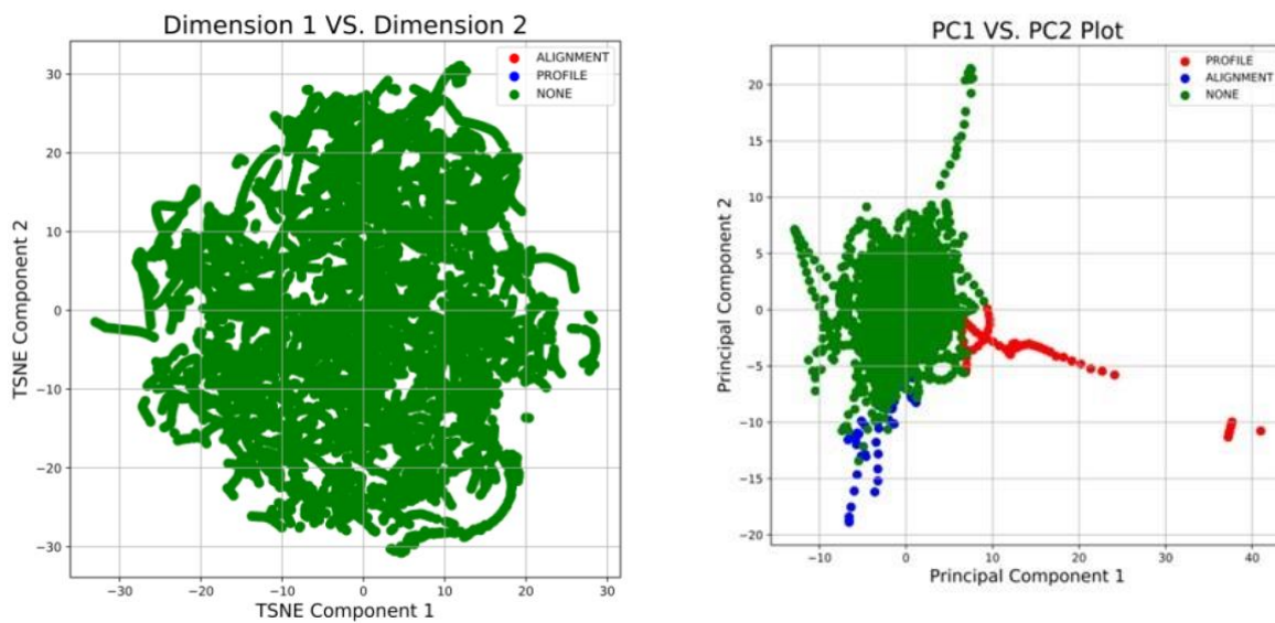
Figure 9 (a) Principal component defects plot, (b) TSNE 2D plot.
